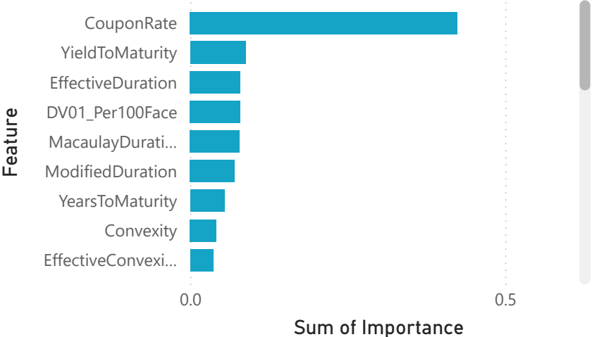
Top Features Influencing Bond Price
